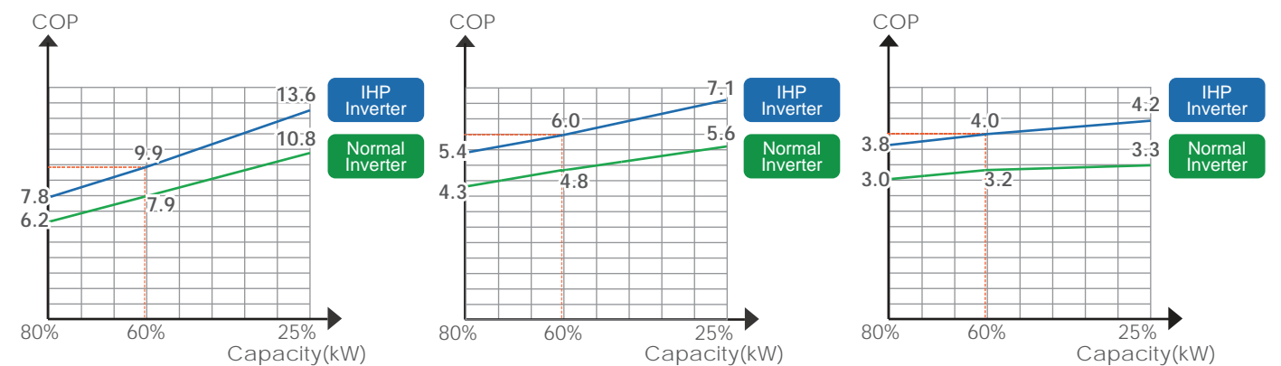
Performance condition: Air 27°C/Water 26°C/Humidity 80% Performance condition: Air 15°C/Water 26°C/Humidity 70% Performance condition: Air 2°C/Water 26°C/Humidity 80%
