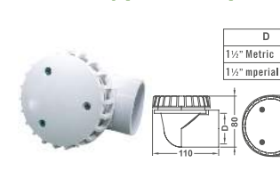
Ø2 Section Drain Ell Body(Threated)
