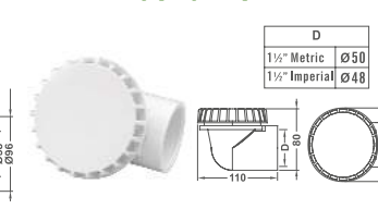
Ø2 Section Drain Ell Body(Slip Fit)
