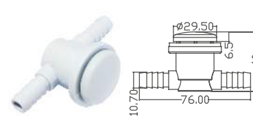
Twin Hole Air Jet
