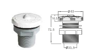
Standard Air Control
