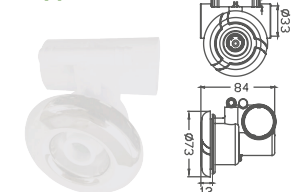
I Type Jet
