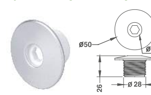
Ø2" Face (Standard) Jet
