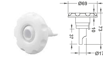
Ø2-3/4" Face Eyeball Spa Jet
