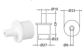
Barb Plug
