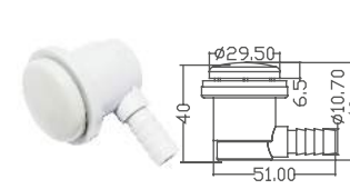
Single Hole Air Jet
