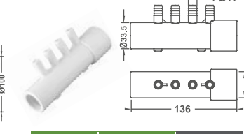
Port Air Manifold
