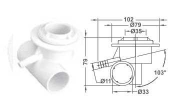
Ø10mm Barb Air & Ø25mm Water
