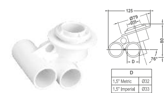
Ø25mm Barb Air & Ø25mm Water Tee Body
