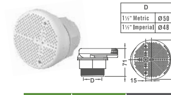
Ø2 Section Drain Lock Nut
