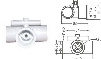
Tiny Air Jet
