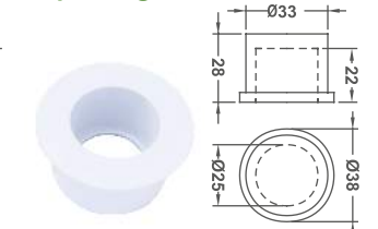
Pipe Plug
