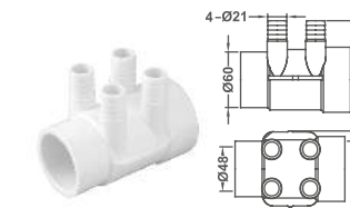
Port Water Barb Manifold
