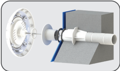
Concrete Pool+Liner
