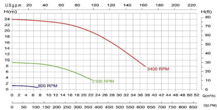
EPV300 Pump Curve
