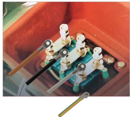
3 phase power 4 wires power line connection
