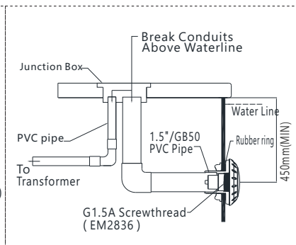
4) TOP13-EM(Vinyl Pool/Fiberglass Pool)
