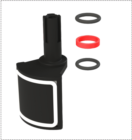
8. Diverter module Includes 2 shaft O-ring and 1 washer
