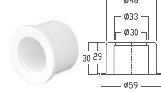
Pipe Plug
