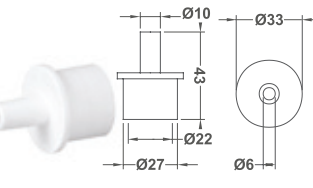
Barb Plug
