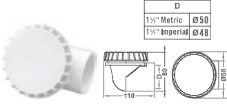
φ2 Section Drain EII Body(Slip Fit)
