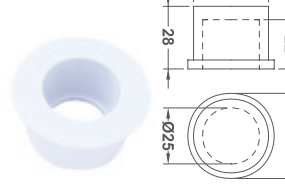
Pipe Plug
