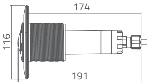
Suction Fittings
