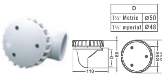
φ2 Section Drain EII Body(Threaded)
