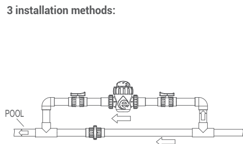
Horizontal Installation
