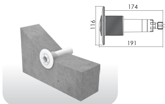
Suction Fittings
