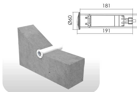
1.5" PVC Pipe
