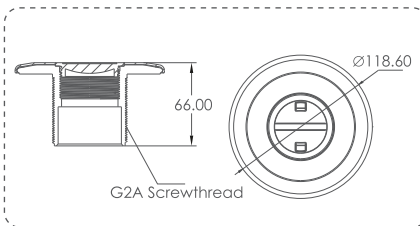
Vacuum Fitting (EM2831) (Concrete Pool)
