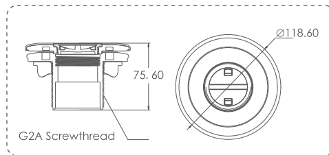
Vacuum Fitting (EM2836) (Vinyl Pool)
