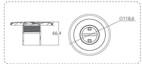
Vacuum Fitting (EM2848) (Concrete Pool)
