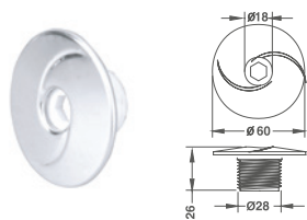
φ2" Face (Spiral) Jet
