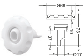
φ2-3/4" Face Eyeball Spa Jet
