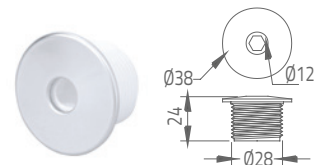
φ1-1/2" Face (Standard) Jet
