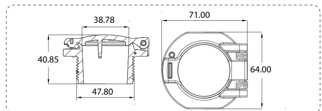
Vacuum Lock Safety Wall Fitting (EM2855)
