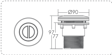
Vacuum Fitting (EM2827V) (Vinyl Pool)
