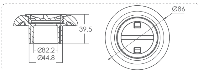
Vacuum Fitting (EM2857E) (Concrete Pool)
