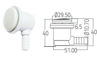
Single Hole Air Jet
