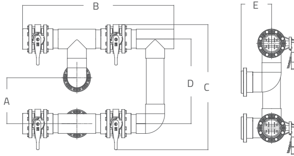
4 Way Butterfly Valve NBV30-NBV80
