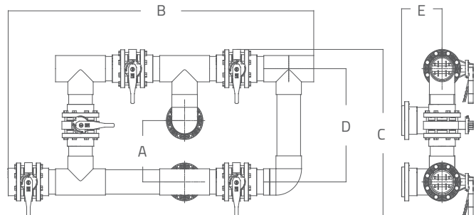
5 Way Butterfly Valve NBV30-NBV80
