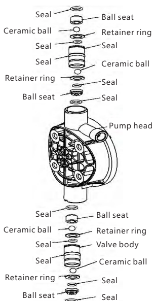
Fig 1: Exported diagram of the pump base
